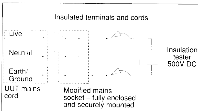
Figure 1.1: Test adaptor
